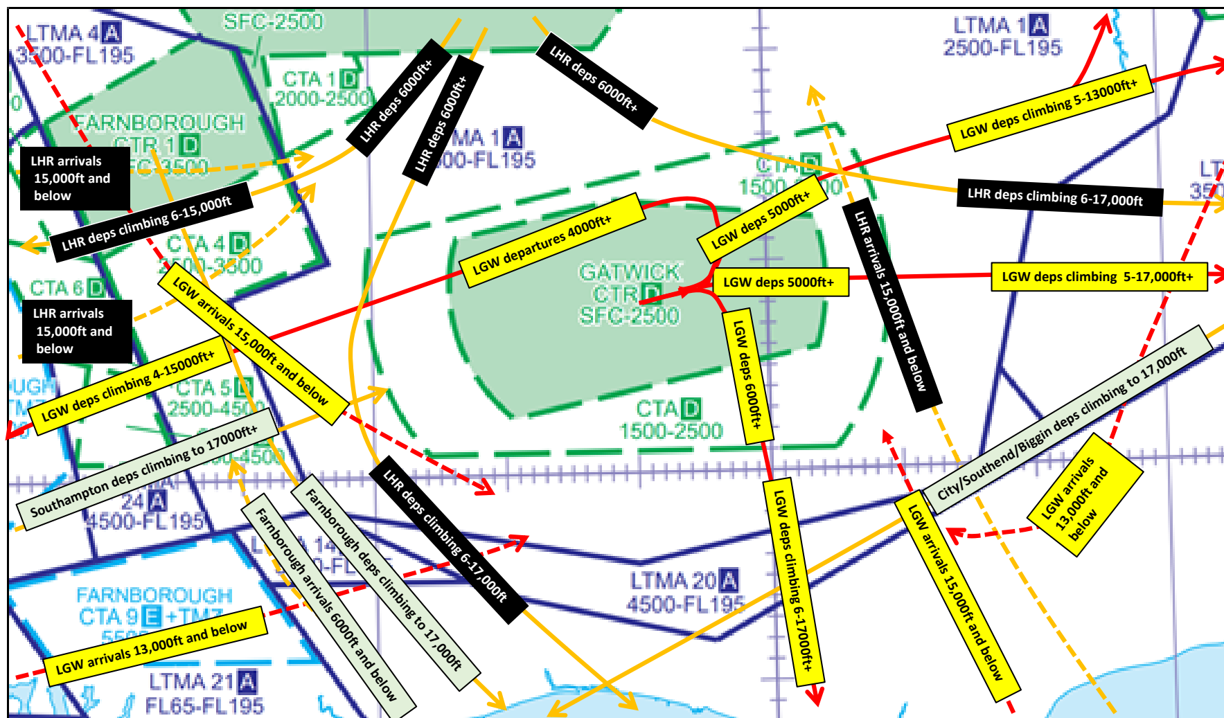
Figure 28 Diagrammatic representation of interdependencies between Gatwick (example for easterlies) and other TMA airport traffic flows
